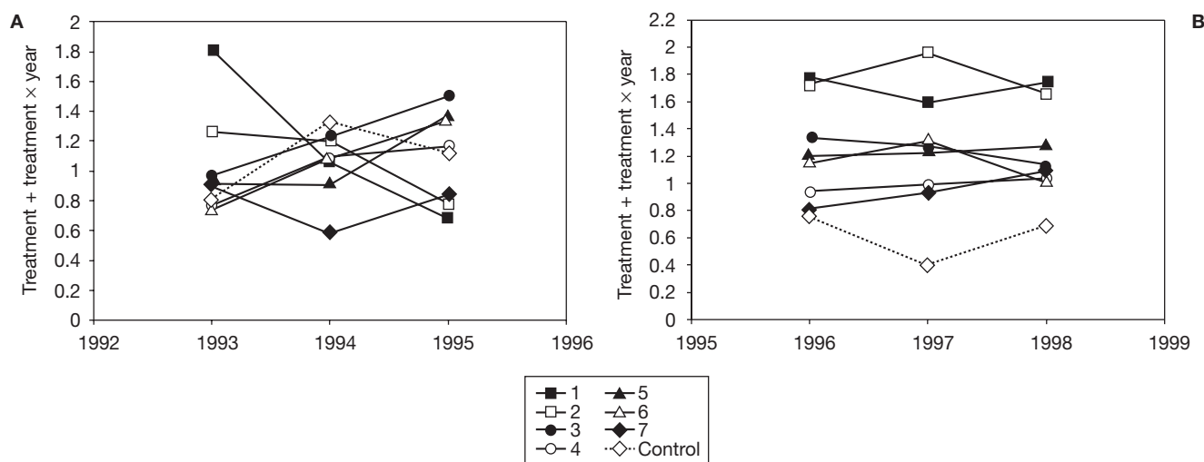
Figure 2. Time trends for treatment BLUE + treatment \times year BLUP. A) Data-series 1993-1995; B) Data series 1996-1998.
